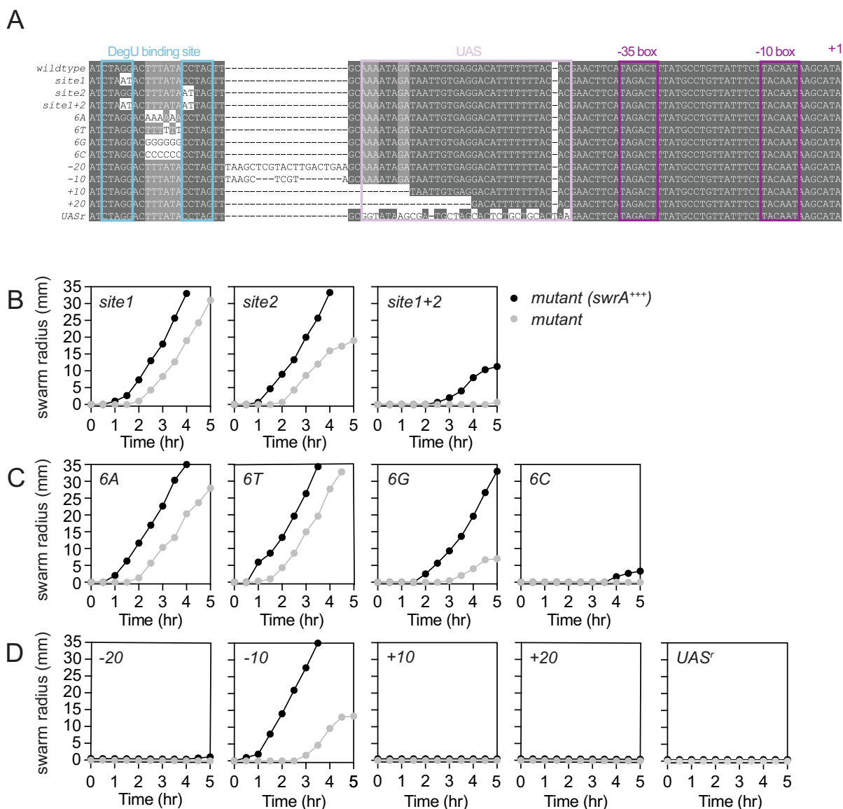
Figure 6. The distance between the DegU binding site and the P_{flache} promoter is important for activation. A) Alignment of P_{flache} promoter mutations used in the assay below. Blue boxes highlight the location of the 5-8-5 inverted repeat; Pink box highlights the upstream activating sequence; purple highlights that -35 and -10 SigA boxes of the P_{flache} promoter and +1 indicates the transcriptional start site. B) Quantitative swarm expansion assays of strains mutated for the DegU binding site inverted repeat sequences (gray circles), and strains containing the indicated mutations and SwrA overexpressed by IPTG induction ( swrA^{+++} , black circles). The following strains were used to generate this panel: site1 (DB164, DB198), site 2 (DB102, DB197), and site 1+2 double mutant (DB49, DB58). C) Quantitative swarm expansion assays of strains with the indicated sequence between the DegU binding site repeat elements (gray circles), and strains containing the indicated sequence and SwrA overexpressed by IPTG induction ( swrA^{+++} , black circles). The following strains were used to generate this panel: 6A (DB48, DB196), 6 T (DB47, DB228), 6G (DB165, DB199), and 6C (DB166, DB200). D) Quantitative swarm expansion assays of strains in which the 5-8-5 DegU binding site motif was moved farther away (-20 or -10 bp, respectively) or towards (+10 or +20 bp, respectively) the P_{flache} promoter (gray circles), and strains containing the indicated relocation and SwrA overexpressed by IPTG induction ( swrA^{+++} , black circles) The following strains were used to generate this panel: -20 (DB488, DB524), -10 (DB487, DB523), +10 (DB195, DB220), +20 (DB486, DB522) and UAS r (DB1020, DB1071). Each data point is the average of three replicates.
