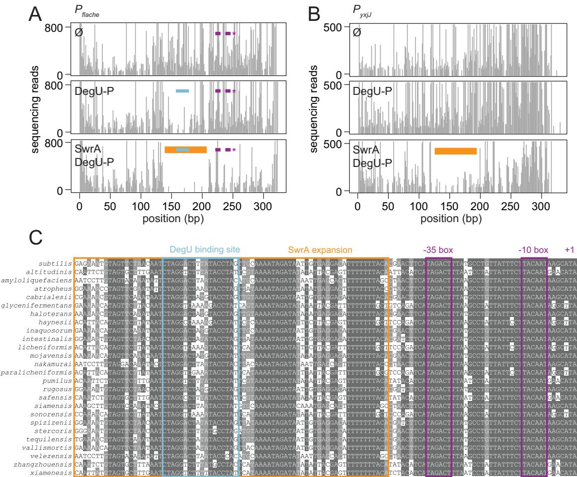
Figure 5. SwrA increases the length of DNA protected by DegU-P. A) DNaseI sequencing footprint analysis of the P flache promoter. 300 bp fragments of dsDNA were fluorescently labeled on the forward strand, the indicated protein was added, followed by partial digestion with DNase I and sequencing of the digested fragments. Top panel, 1 μM BSA added; middle panel 3 μM of DegU-P-His 6 added; bottom panel 3 μM of DegU-P-His 6 and 1 μM of GST-SwrA added. Blue bars indicate the location of the 5-8-5 inverted repeat; orange bars indicate the expanded region of SwrA/DegU-P protection; purple bars indicate the -35 SigA box, the -10 SigA box, and the +1 transcriptional start sites of the P flache promoter are marked with an asterisk. Peaks indicate the number of sequence reads terminating at that location on one strand. B) DNaseI sequencing footprint analysis of the P yxjJ promoter. Top panel, 1 μM BSA added; middle panel 3 μM of DegU-P-His 6 added; bottom panel 3 μM of DegU-P-His 6 and 1 μM of GST-SwrA added. Peaks indicate the number of sequence reads terminating at that location. The location of the promoter and transcriptional start site for P yxjJ is unknown. C) Alignment of the P flache promoter fragment. Blue boxes highlight the location of the 5-8-5 inverted repeat (repeat sequences in bold); Orange box highlight the expanded region of SwrA/DegU-P protection; purple highlights the -35 and -10 SigA boxes of the P flache promoter and +1 indicates the transcriptional start site.
